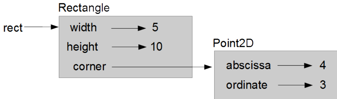
Figure 12.2: Object diagram.
