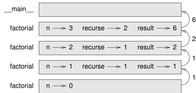
Figure 5.1: Stack diagram.
