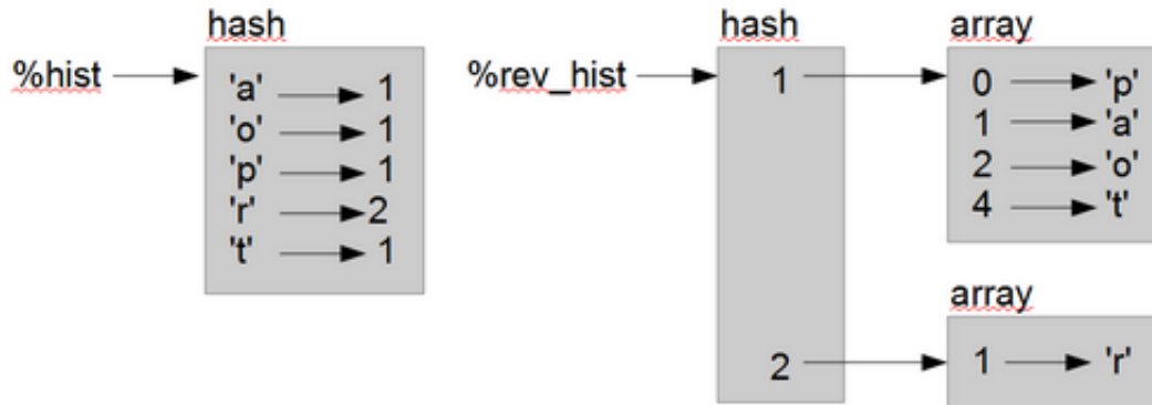
Figure 10.1: State diagram.
