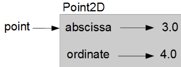
Figure 12.1: Object diagram.
